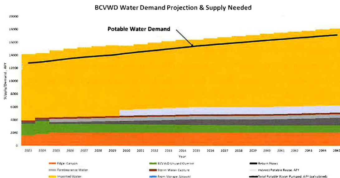
Figure 8: BCVWD's Water Supply and Demand Projection to 2045
