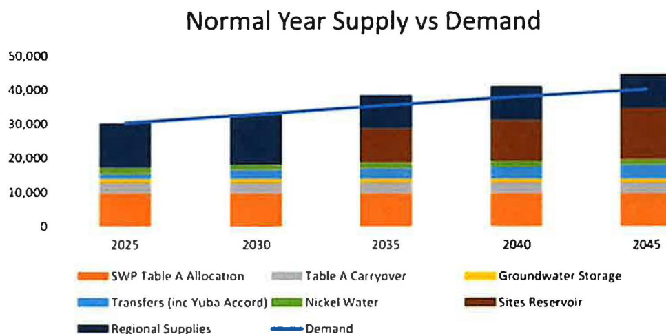
Figure 6: SGPWA's Water Service Reliability through 2045 (AFY)
